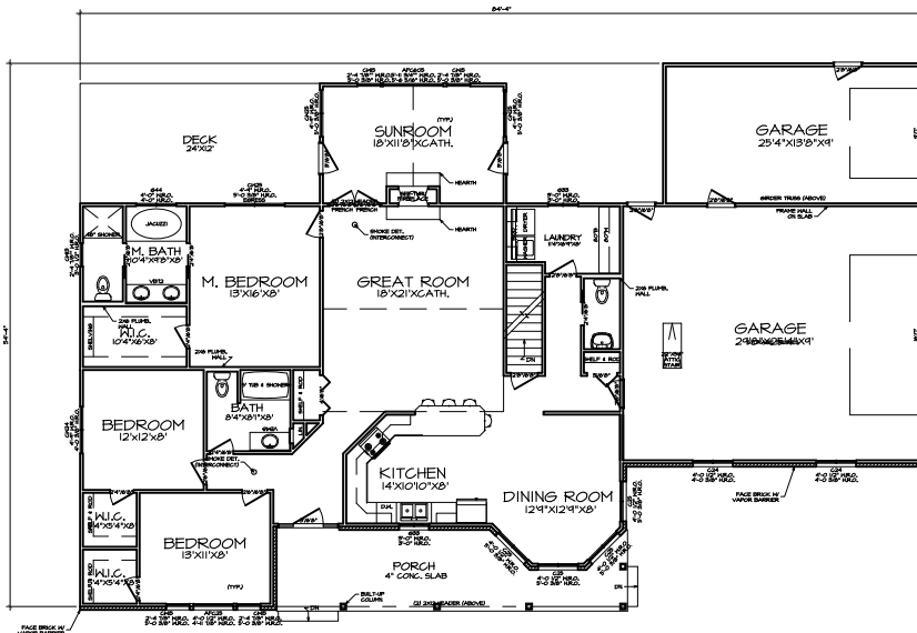
1 FIRST FLOOR PLAN A-5
